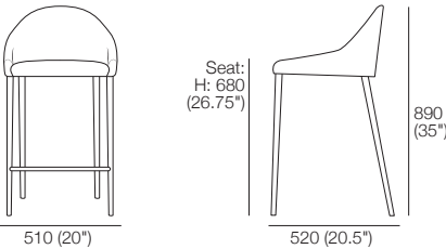
Counter Stool (Upholstered) Front View | Side View
