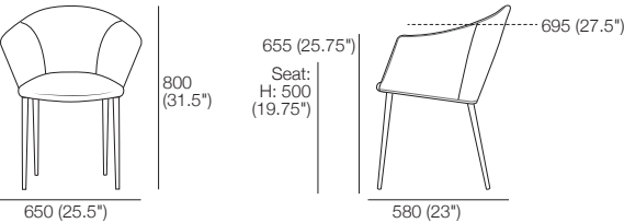
Dining Chair (Upholstered) Leather Detail Indicated Front View | Side View
